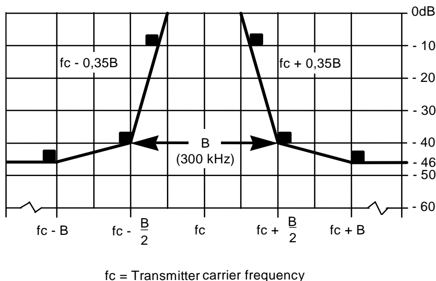
Figure 3: Spectral mask for analogue or digital modulation with B = 300 kHz
